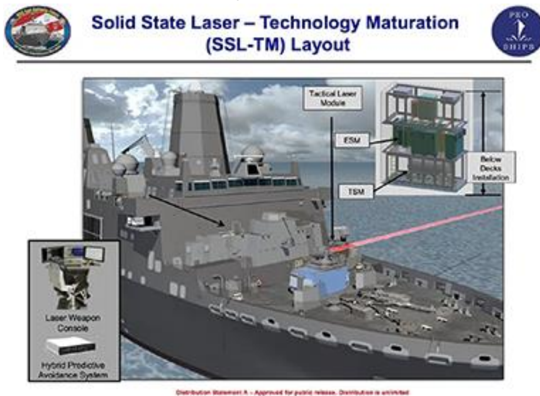
Figure 5. Navy Graphic of SSL-TM Laser System
